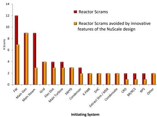
Fig. 1. Number of 2015 reactor scrams expected to be precluded by the NuScale design
