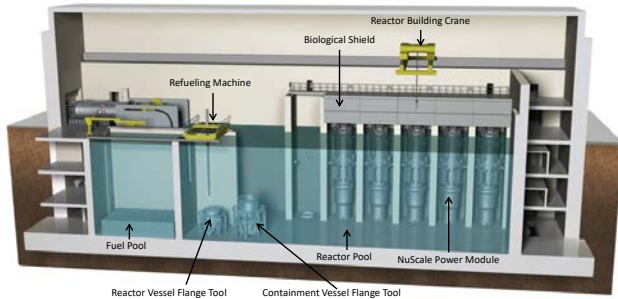
Fig. 1. A 12-Module NuScale reactor building houses the NuScale power modules, fuel pool, and ultimate heat sink for safety.
